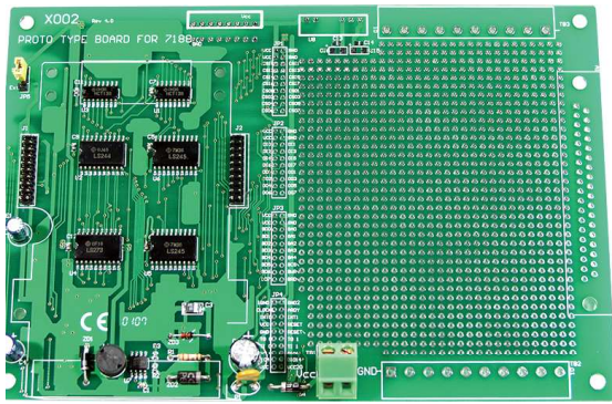
X002 Prototype board
